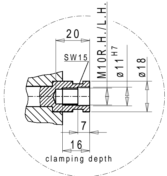
Shank receptacle M10 plan
