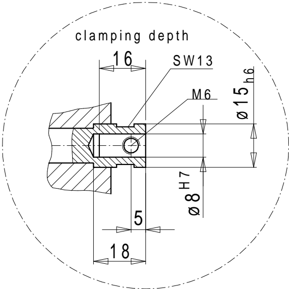
Shank receptacle \varnothing 08H7
