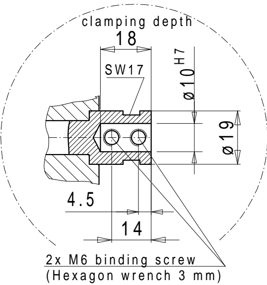
Shank receptacle \varnothing 10H7
