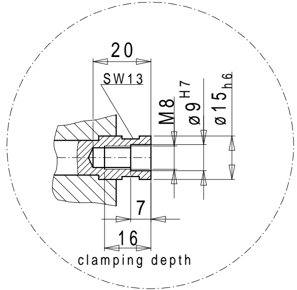
Shank receptacle M08 plan
