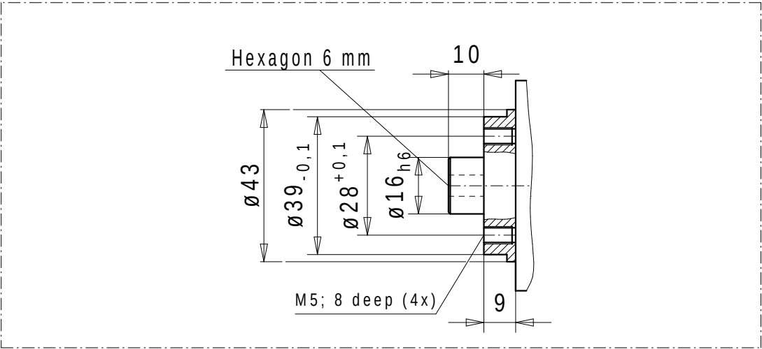
Milling receptacle \varnothing 16h6 \times 10
