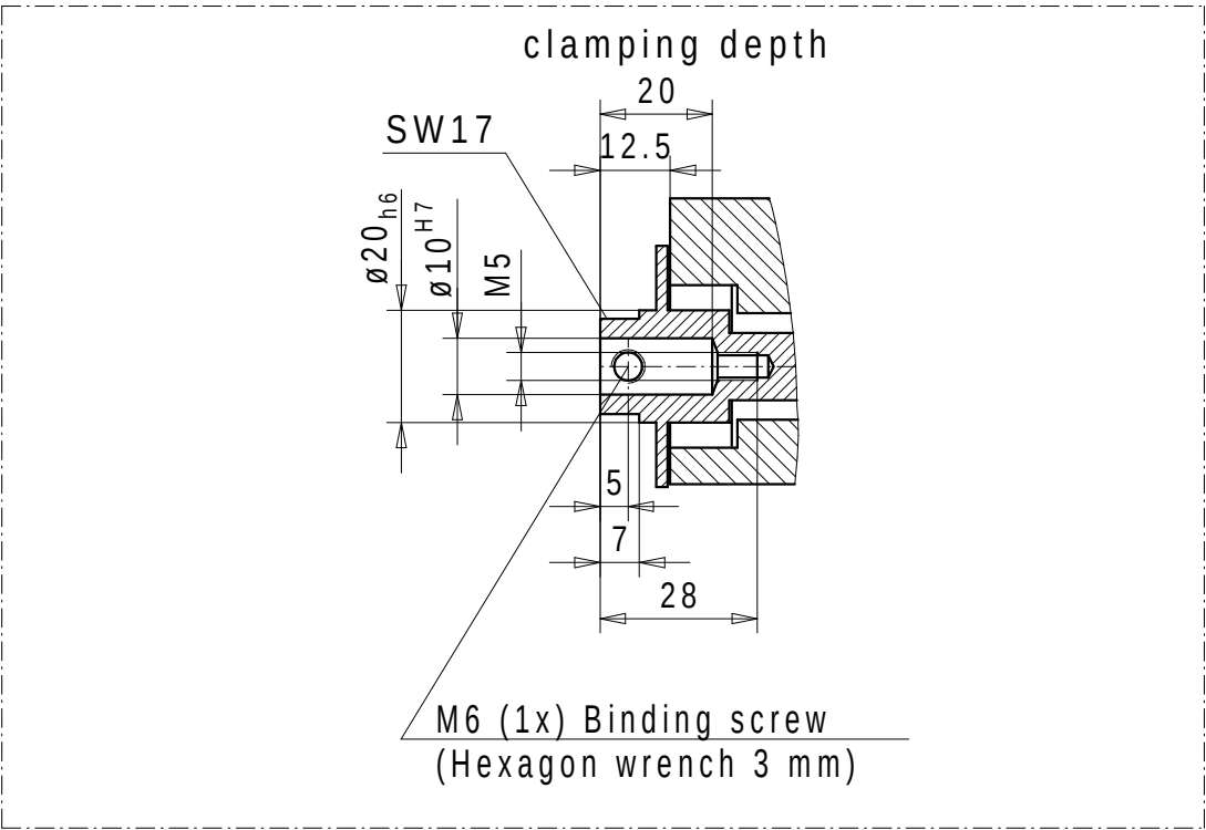
Shank receptacle \varnothing 10H7
