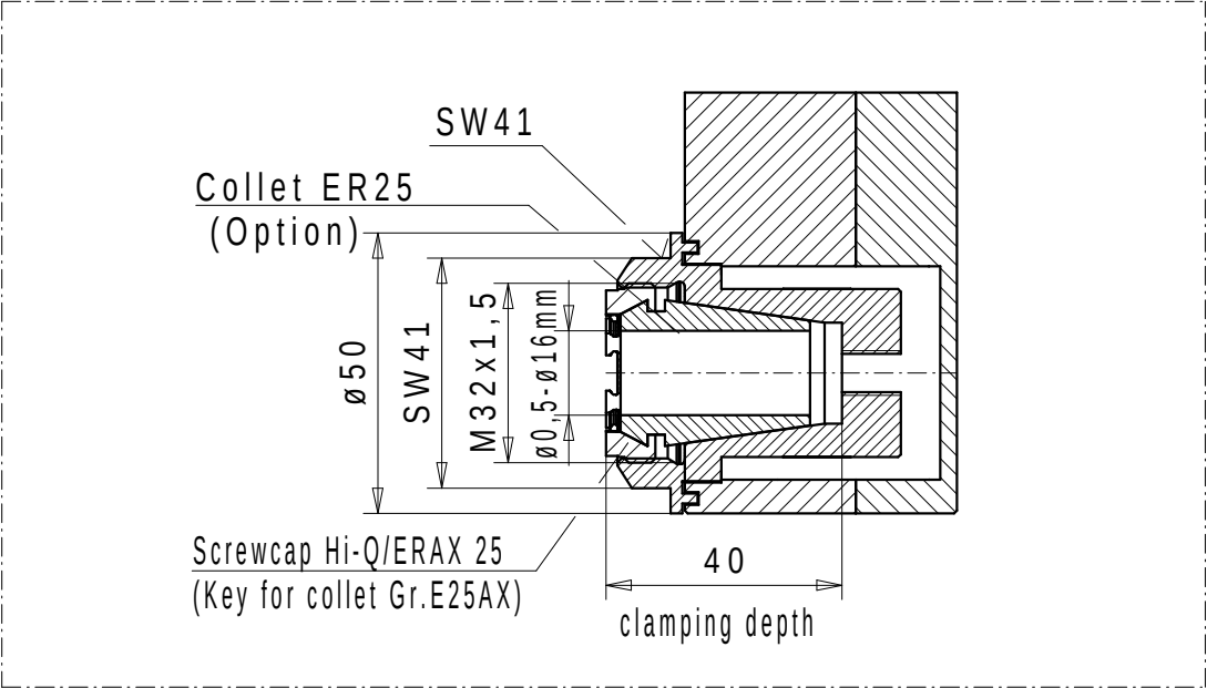
Collet receptacle Hi-Q/ERAX 25 with internal thread
