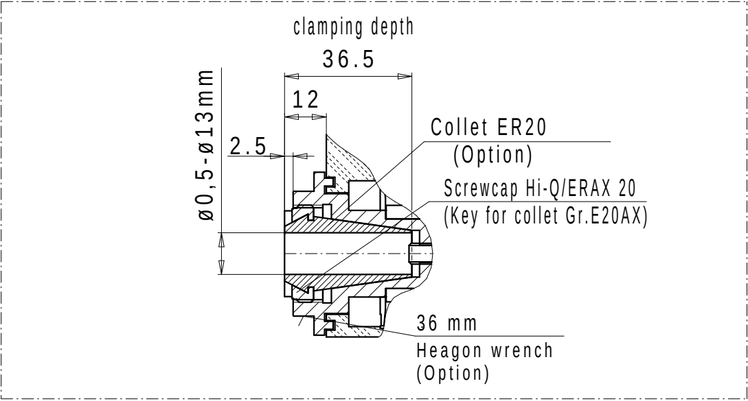
Collet receptacle Hi-Q/ERAX 20 with internal thread
