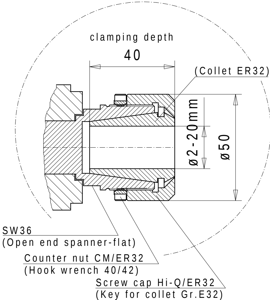
Collet receptacle Hi-Q/ER32
