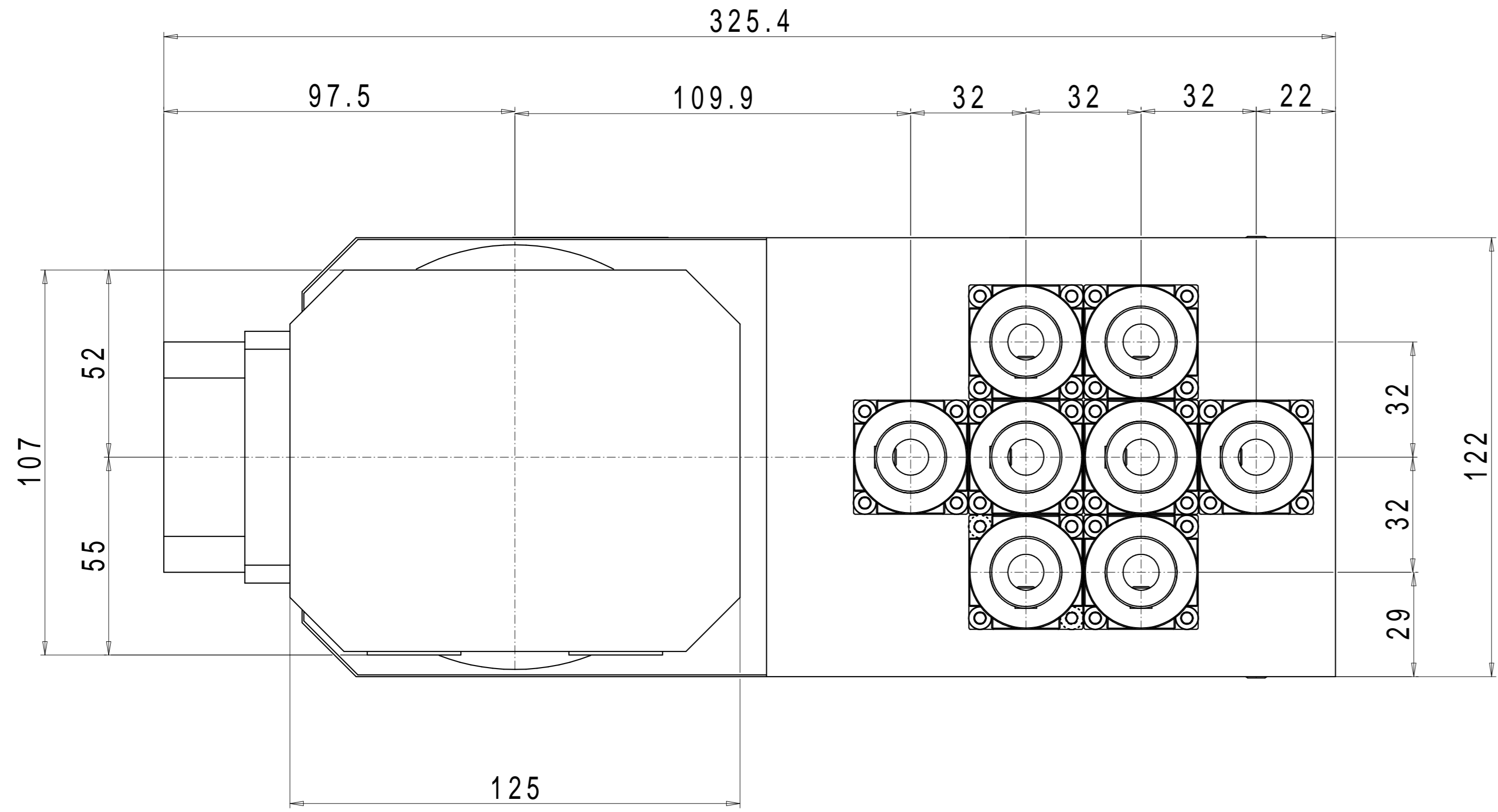
Vertical-Shank receptacle \varnothing 10H7-RE
