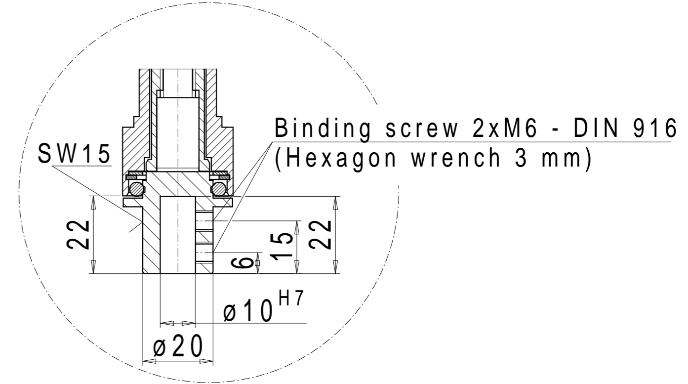
Vertical-Shank receptacle \varnothing 10H7-RE
