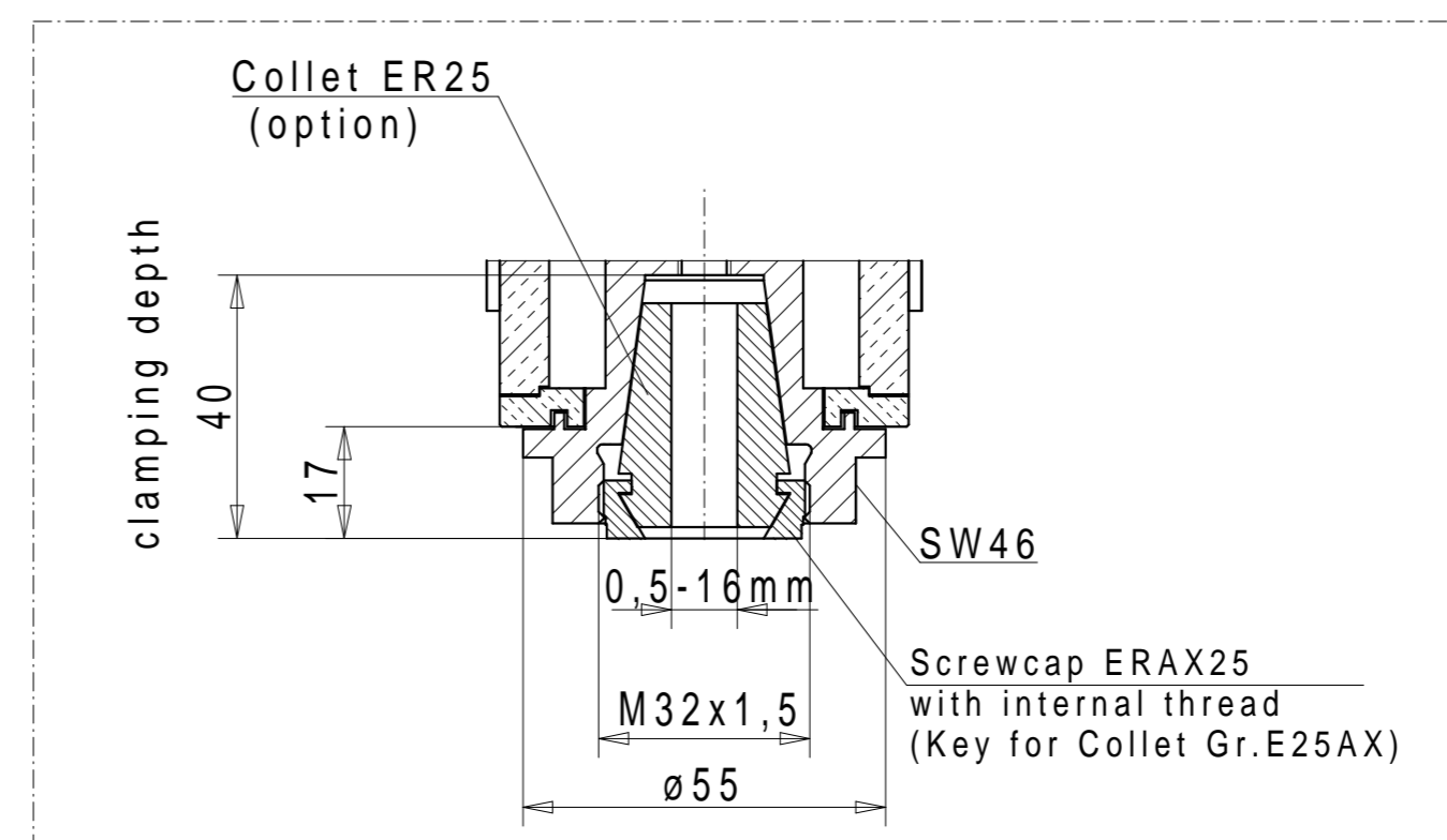
Collet receptacle HI-Q/ERAX25 with internal thread
