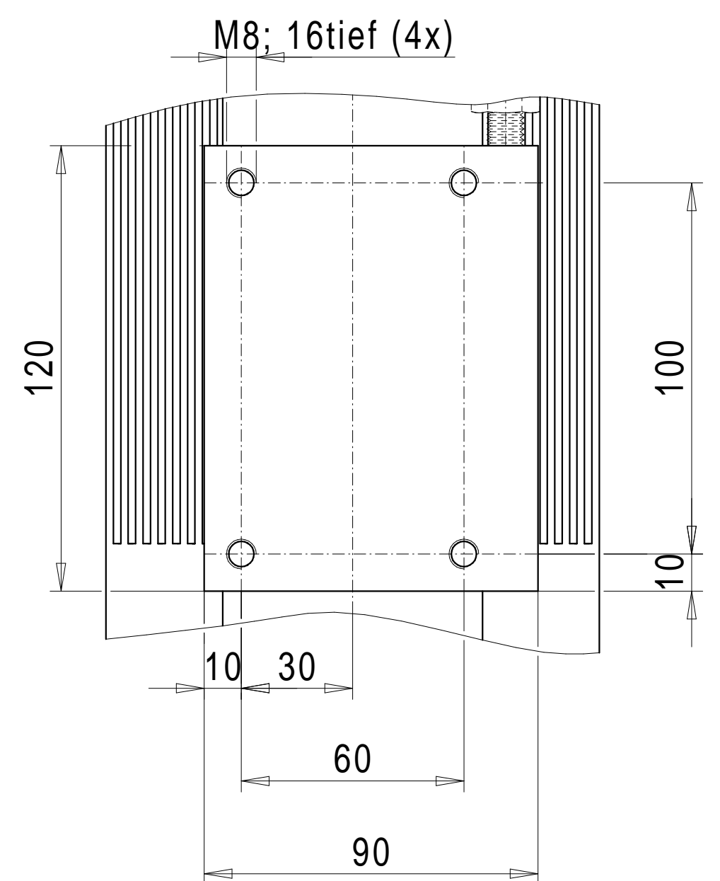
View A-A Clamping piece
