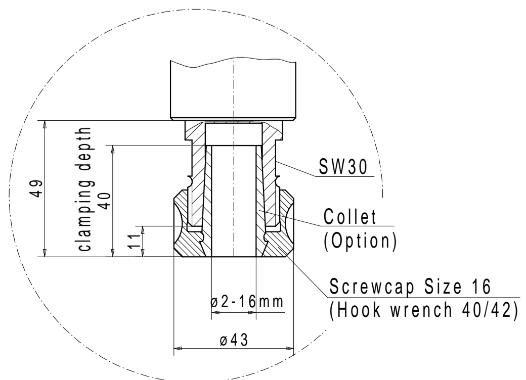
Collet receptacle Size 16
